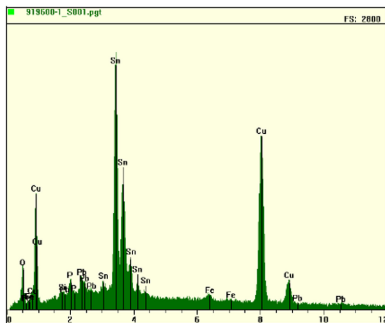
Figure 1: EDS spectrum of shiny surface
