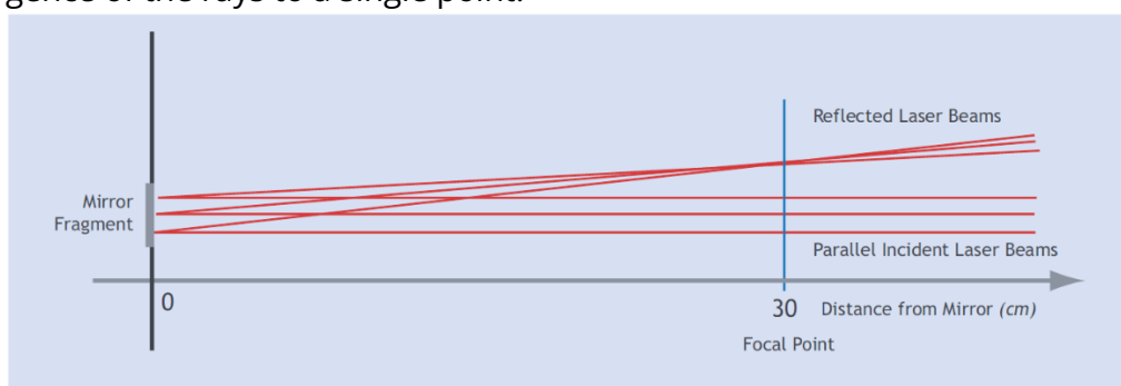
Diagram to show convergence of incident rays reflected from a mirror fragment from Leckie broch stored at the Hunterian Museum, Glasgow.
