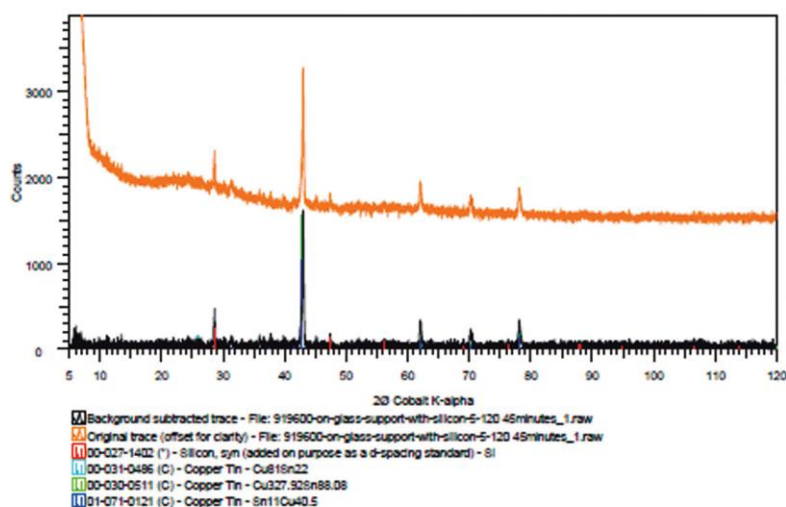
Figure 2: XRD Patterns
