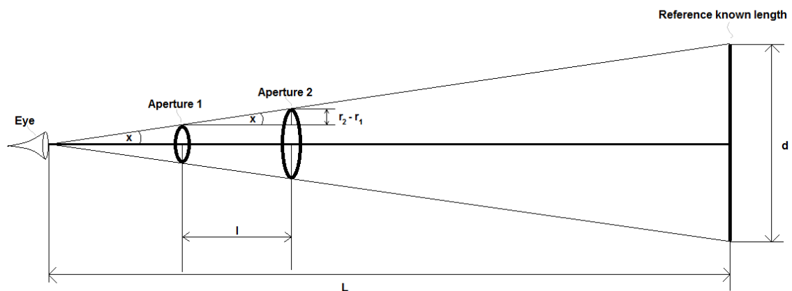
Method of Determining distance L between the eye and a known reference length d (measured in Roman Cubits or Roman Feet) using the Roman Dodecahedron as a dioptron or rangefinder. The Dodecahedron is fixed and the eye is positioned so that the two aperture circumferences appear to coincide with each other. A known measurement length is then moved away from the viewer in a straight line until the ends of the length coincide with the line of sight of the aperture holes. The distance between the eye and the reference length can then be calculated as L = d / (2 \times (r_2 - r_1) / l)
